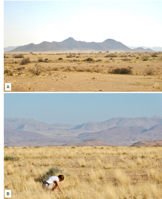
Figure 3: (A) Typical study site in the pre-Namib desert of western Namibia with small trees and bushes. Farm Sphinxblick, 19 June 2005. (B) Setting up traps near the perches on low bushes. 23 November 2009.
