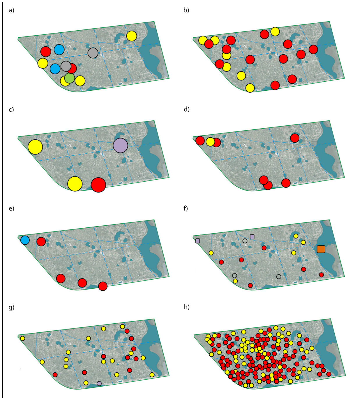
Figure 5: Distribution of breeding pairs/occupied territories of selected bird species in the Ogongo Game Park in 2012. a) Little Bee-eater (yellow), Swallow-tailed Bee-eater (green), Woodland Kingfisher (blue), Pied Kingfisher (grey) and Purple Roller (red);
