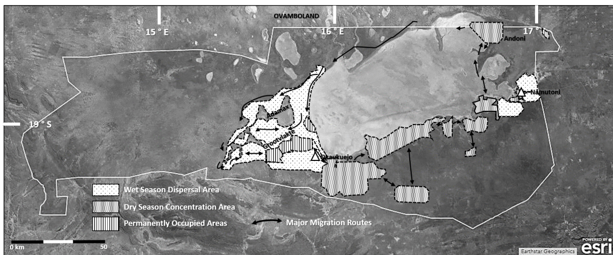
Figure 5: Plains zebra distribution and migration. Based on Ebedes (1976, p. 103).
